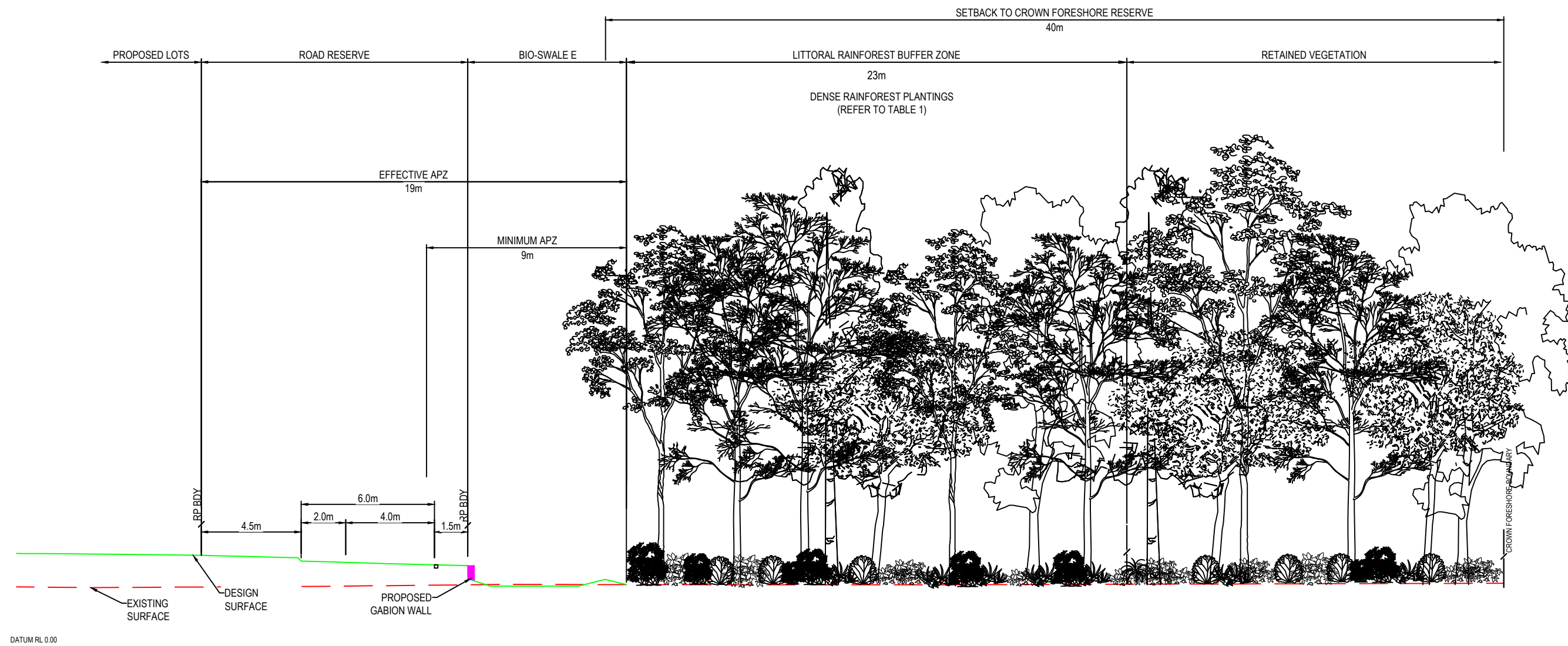
SECTION C - ROAD 02 EVANS RIVER FORESHORE INTERFACE
