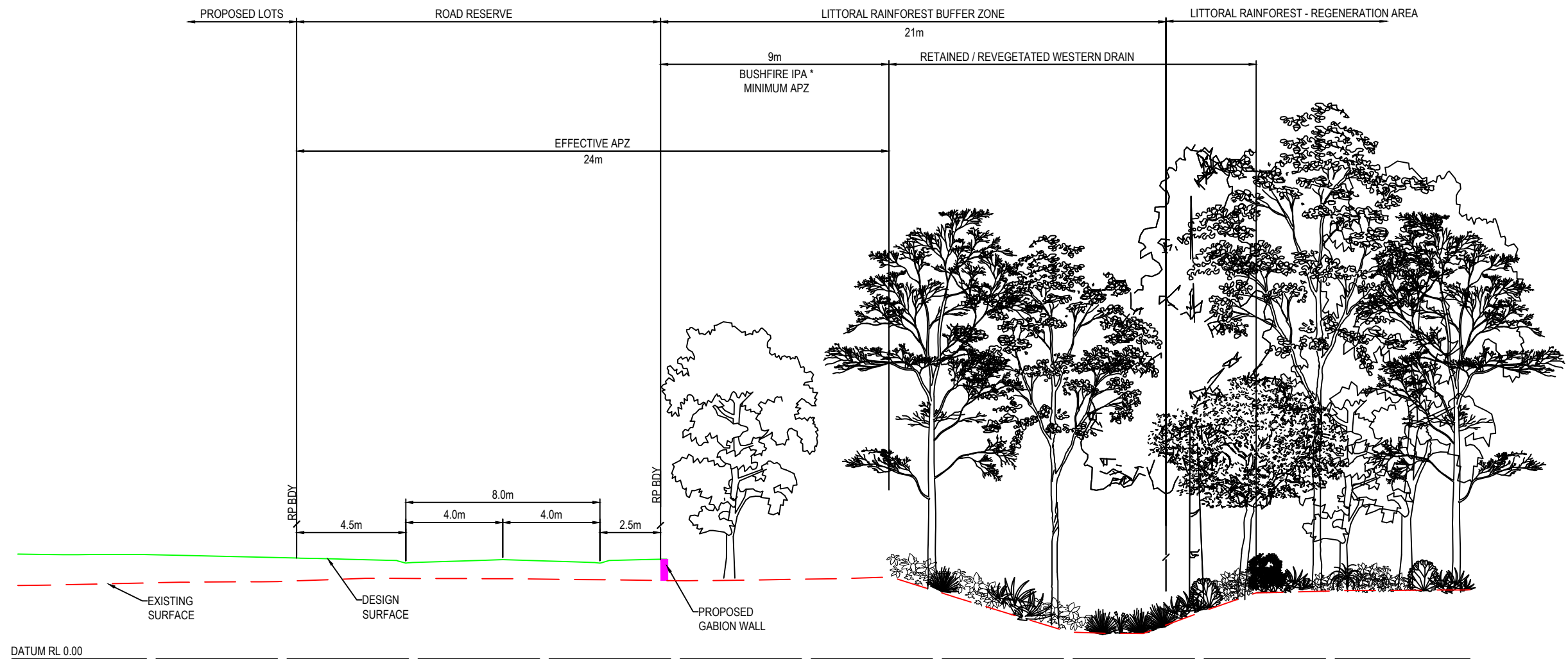
SECTION B - ROAD 03 LITTORAL RAINFOREST INTERFACE
