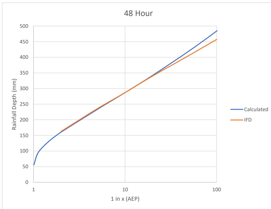
Figure D.3 Gauge 58061 (Woodburn, Cedar Street), 48 hour duration
