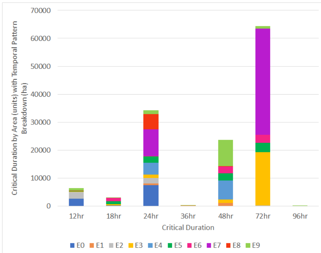
Figure 8.7 Graphical Representation of Event Selection: 2% AEP
