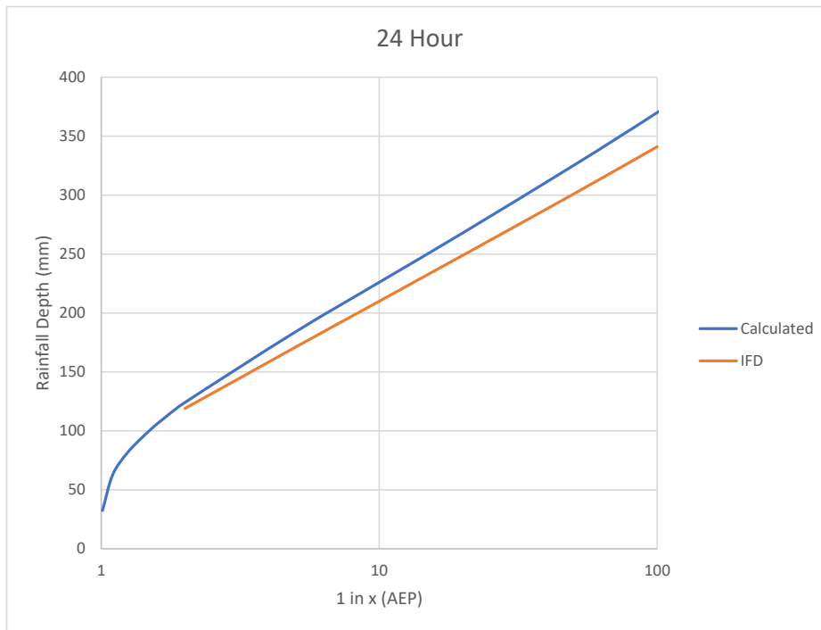
Figure D.6 Gauge 58015 (Coraki, Richmond Terrace), 24 hour duration
