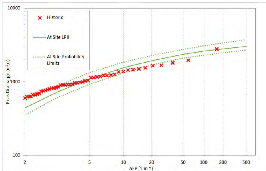
Figure 7.3 Flood Frequency Plot for Kyogle
