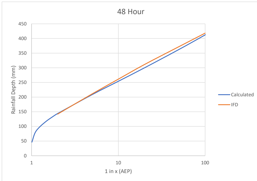
Figure D.31 Gauge 58141 (Loadstone, High View), 48 hour duration
