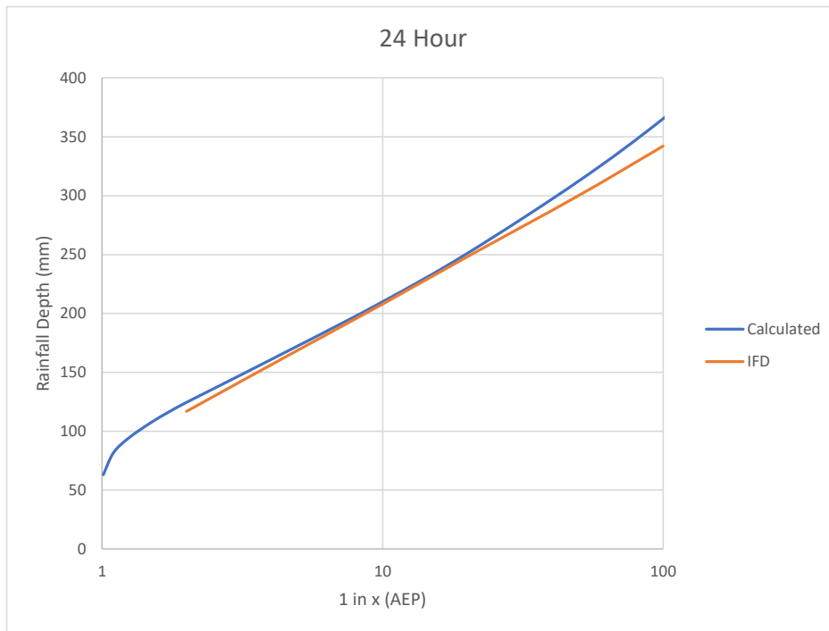
Figure D.12 Gauge 58097 (New Italy Vineyard Haven), 24 hour duration
