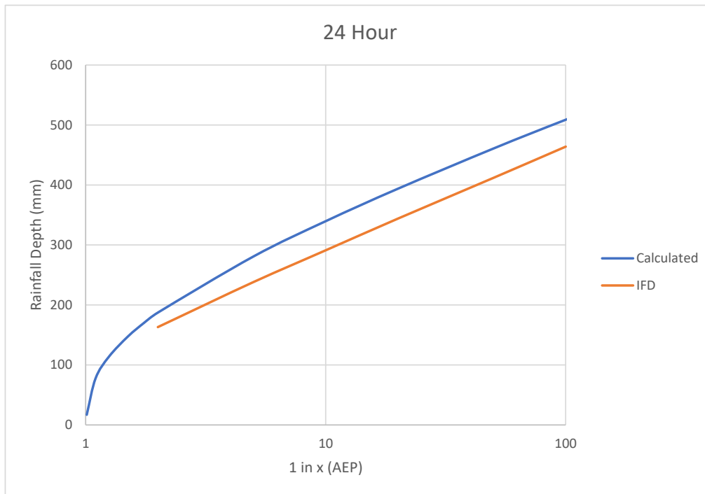
Figure D.20 Gauge 58070 (Rosebank, Repentance Creek), 24 hour duration
