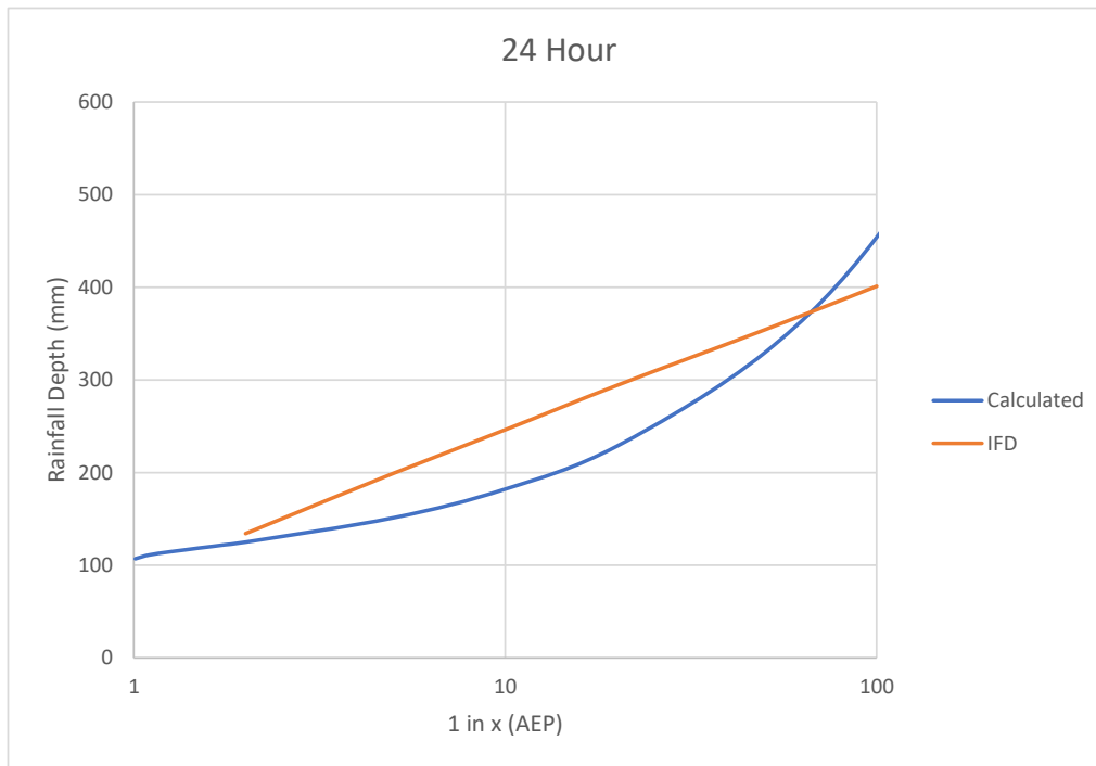
Figure D.4 Gauge 58180 (Nimbin, Goolmangar Creek), 24 hour duration
