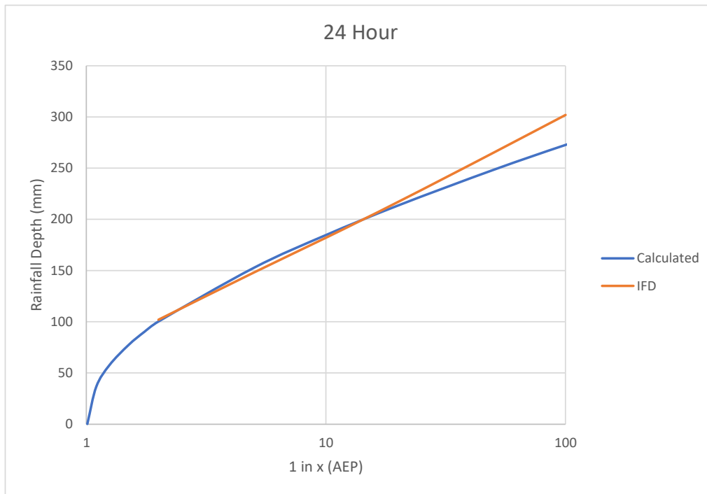
Figure D.26 Gauge 58099 (Whiporie Post Office), 24 hour duration
