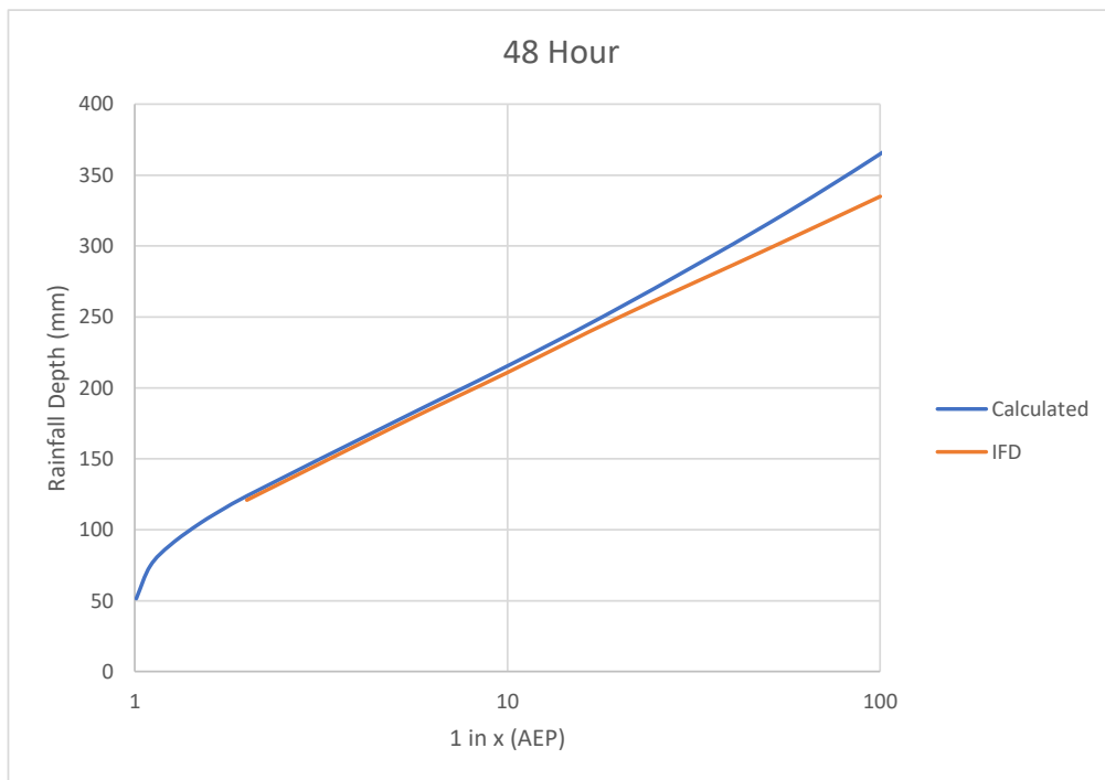
Figure D.17 Gauge 58220 (Woolners Arm), 48 hour duration
