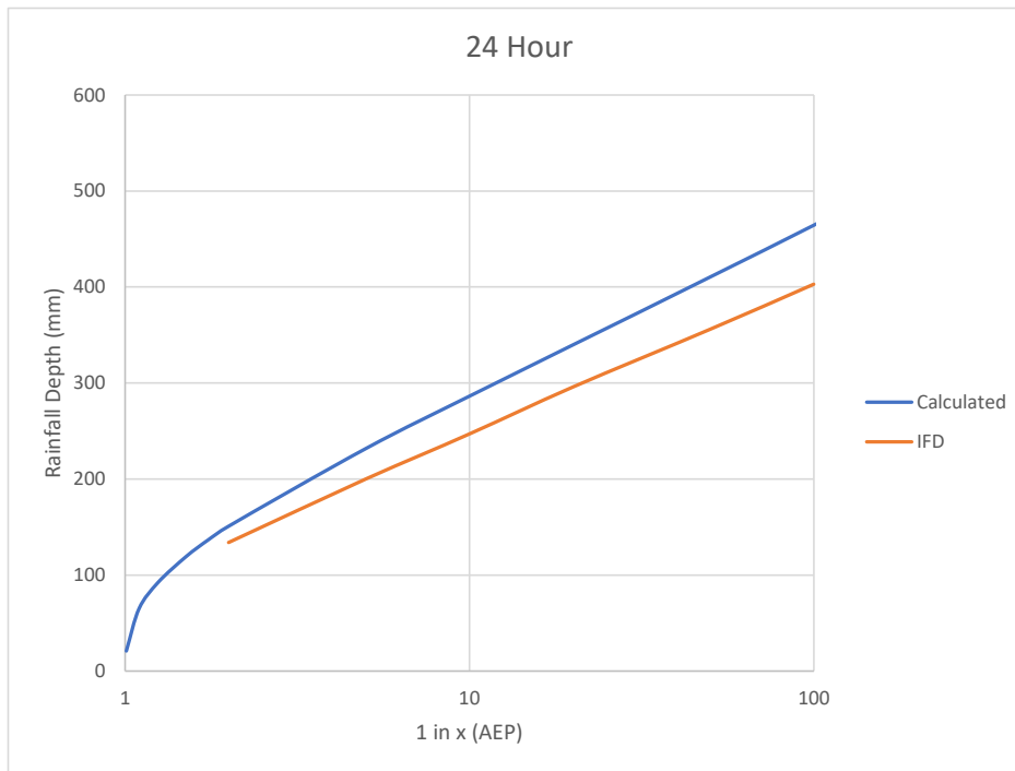
Figure D.8 Gauge 58044 (Nimbin Post Office), 24 hour duration
