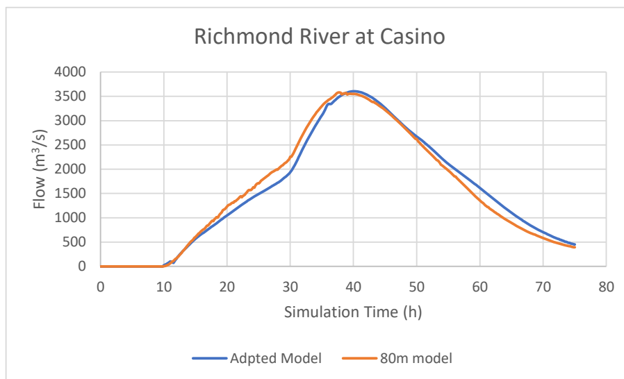
Figure F.1 Comparison at Casino (24h storm duration)
