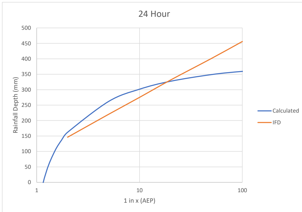
Figure D.28 Gauge 58113 (Green Pigeon, Morning View), 24 hour duration
