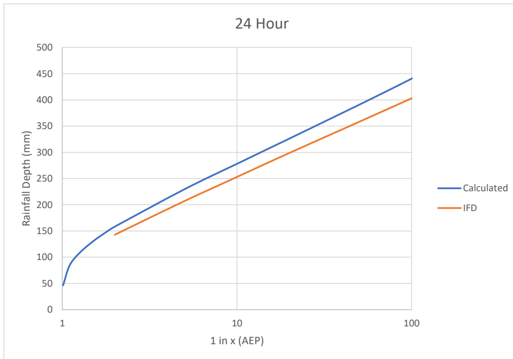
Figure D.22 Gauge 58127 (Clunes, Flatley Drive), 24 hour duration
