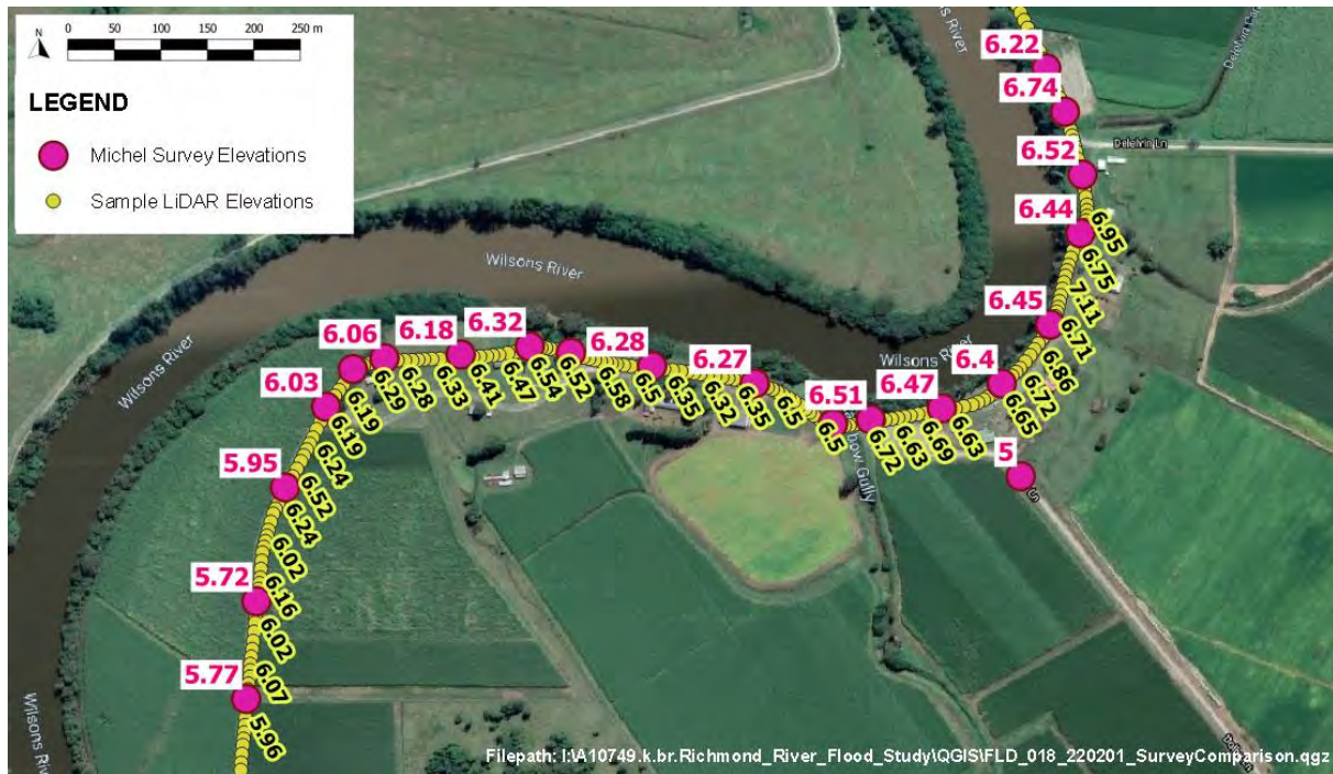
Figure 3.1 Sample showing locations and elevations from Michel Survey (highlighted) versus elevations from LiDAR.
