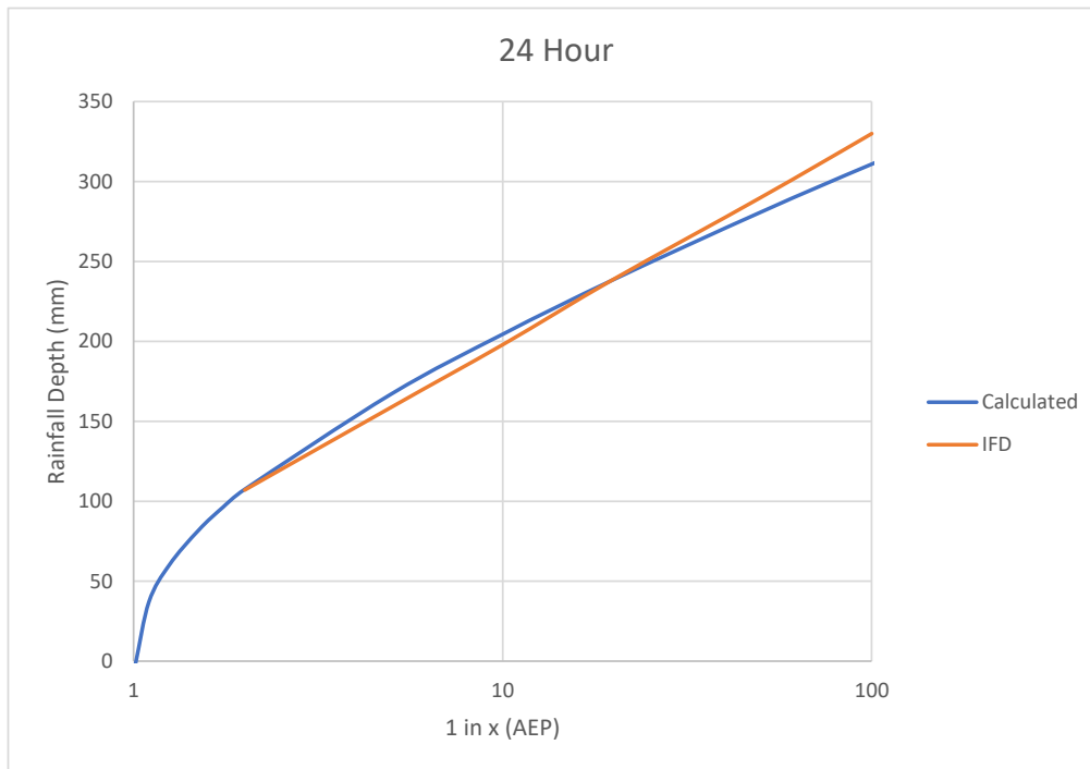
Figure D.30 Gauge 58141 (Loadstone, High View), 24 hour duration
