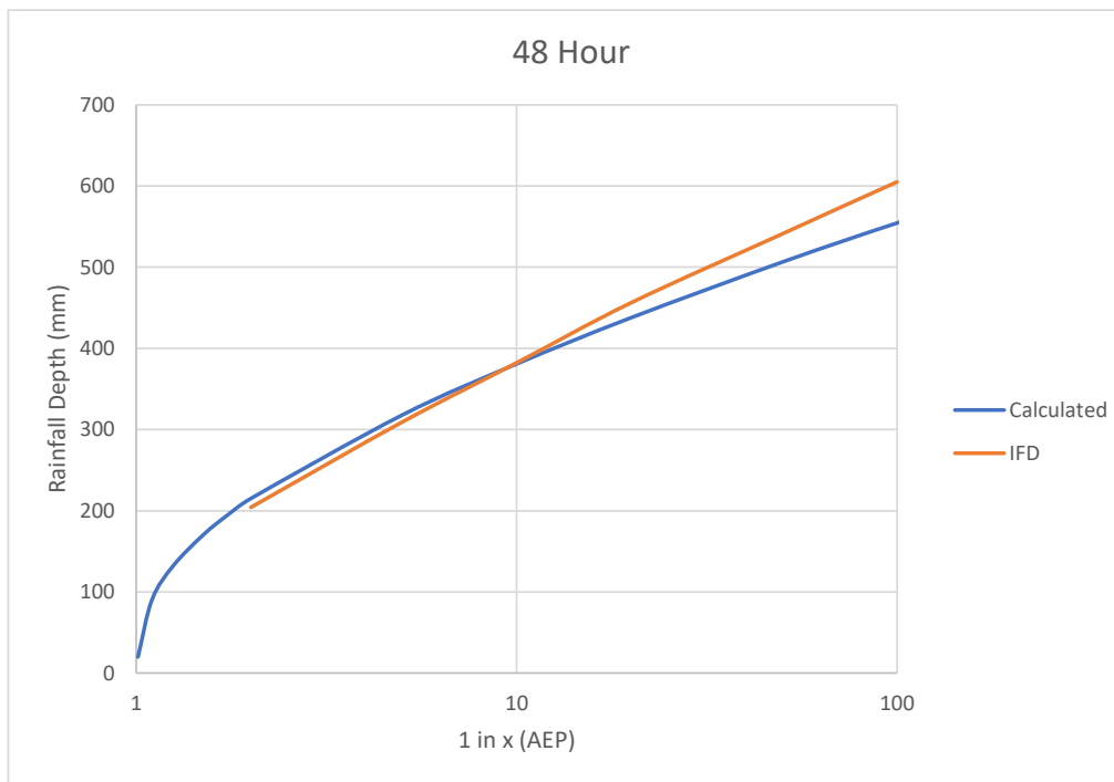
Figure D.25 Gauge 58148 (Lillian Rock, Williams Road), 48 hour duration
