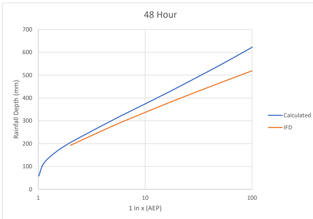
Figure D.23 Gauge 58127 (Clunes, Flatley Drive), 48 hour duration
