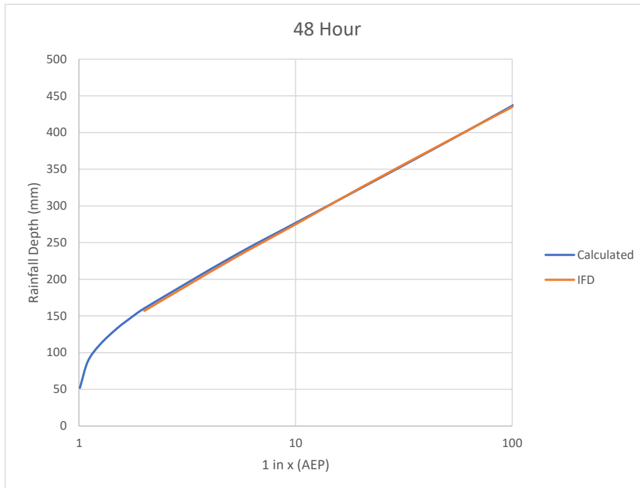
Figure D.7 Gauge 58015 (Coraki, Richmond Terrace), 48 hour duration
