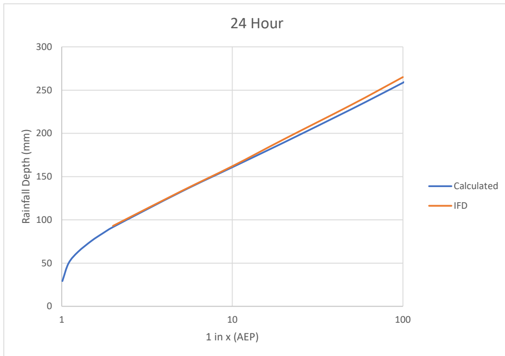
Figure D.16 Gauge 58220 (Woolners Arm), 24 hour duration
