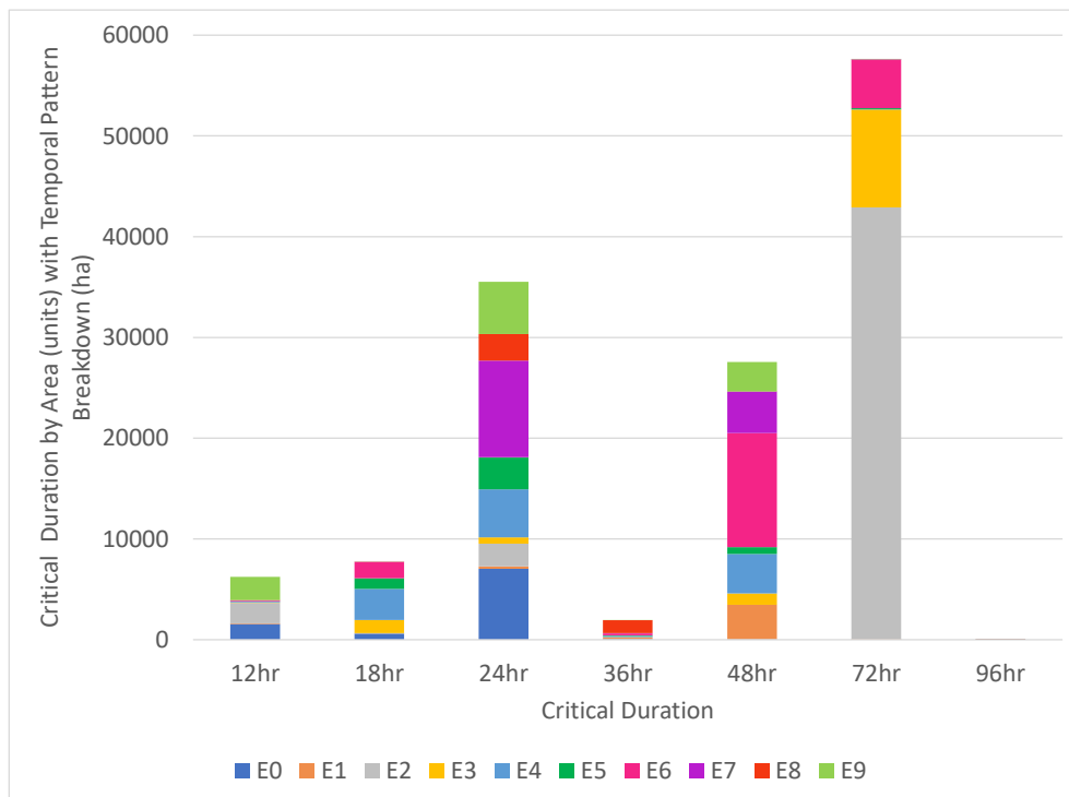
Figure 8.3 Graphical Representation of Event Selection: 1% AEP
