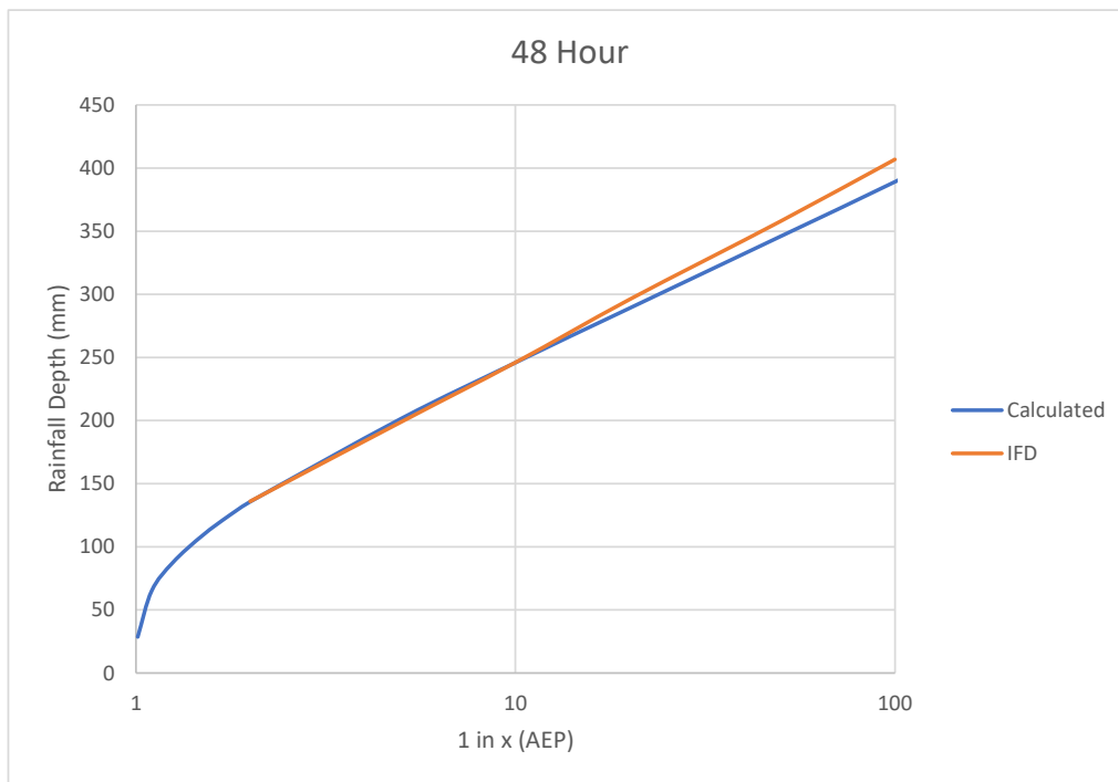
Figure D.27 Gauge 58099 (Whiporie Post Office), 48 hour duration
