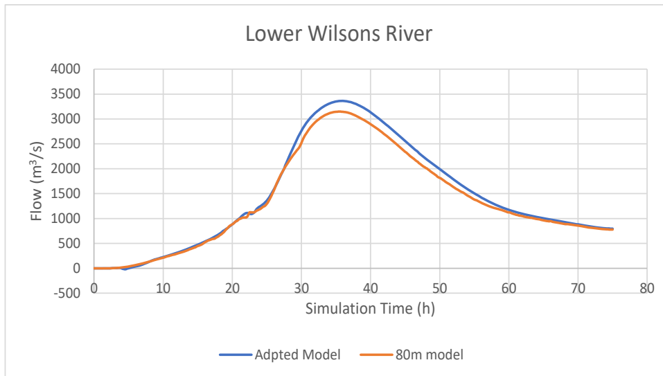
Figure F.3 Comparison on Lower Wilsons River (24h storm duration)
