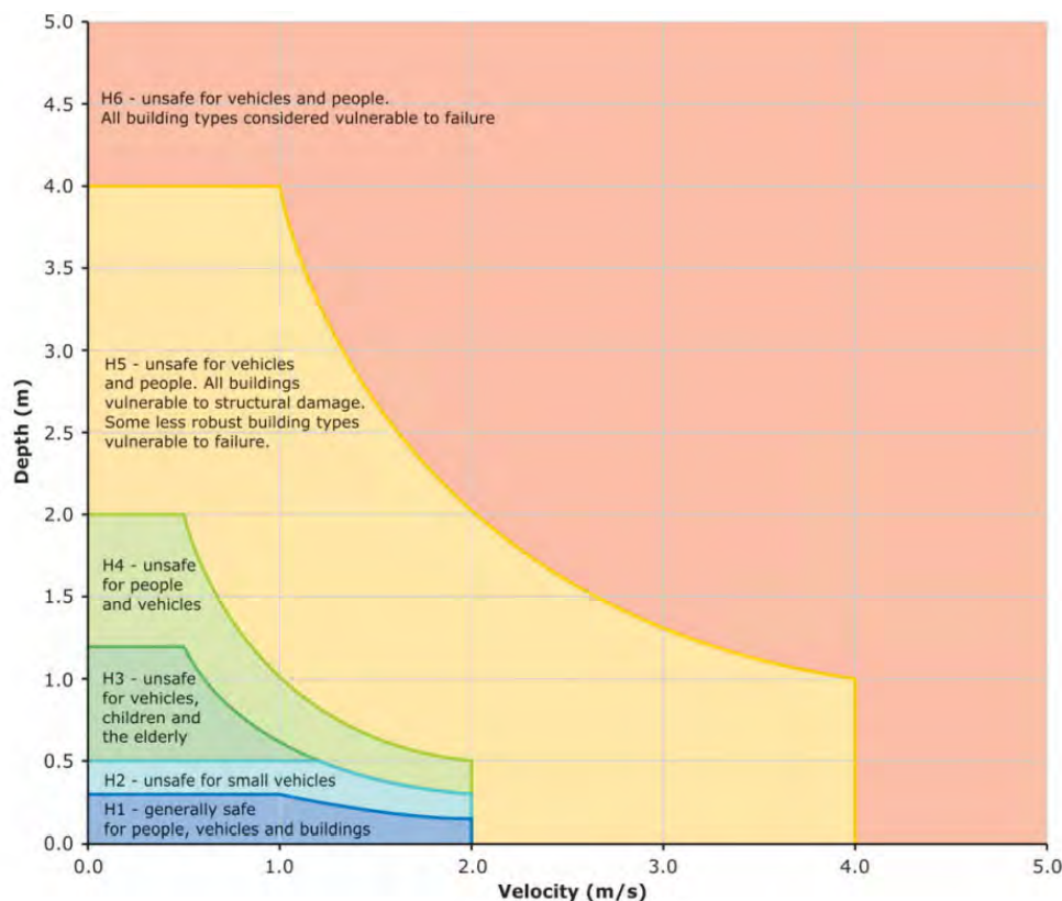
Figure 11.1 General Flood Hazard Vulnerability Curves (AIDR, 2017b)
