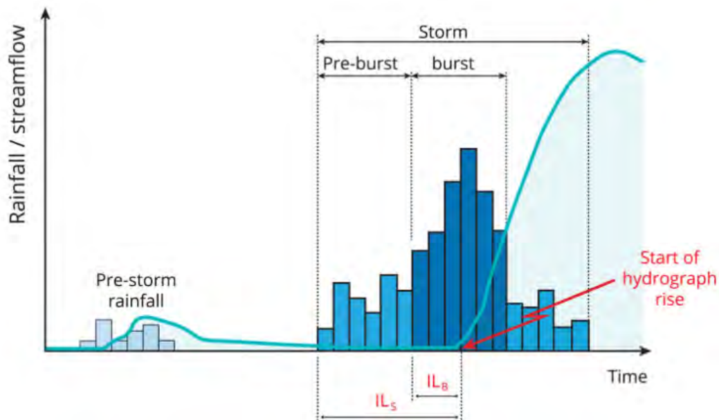
Figure 8.2 Distinction between Storm and Burst Initial Loss (from ARR2016 Book 5, Chapter 3)
