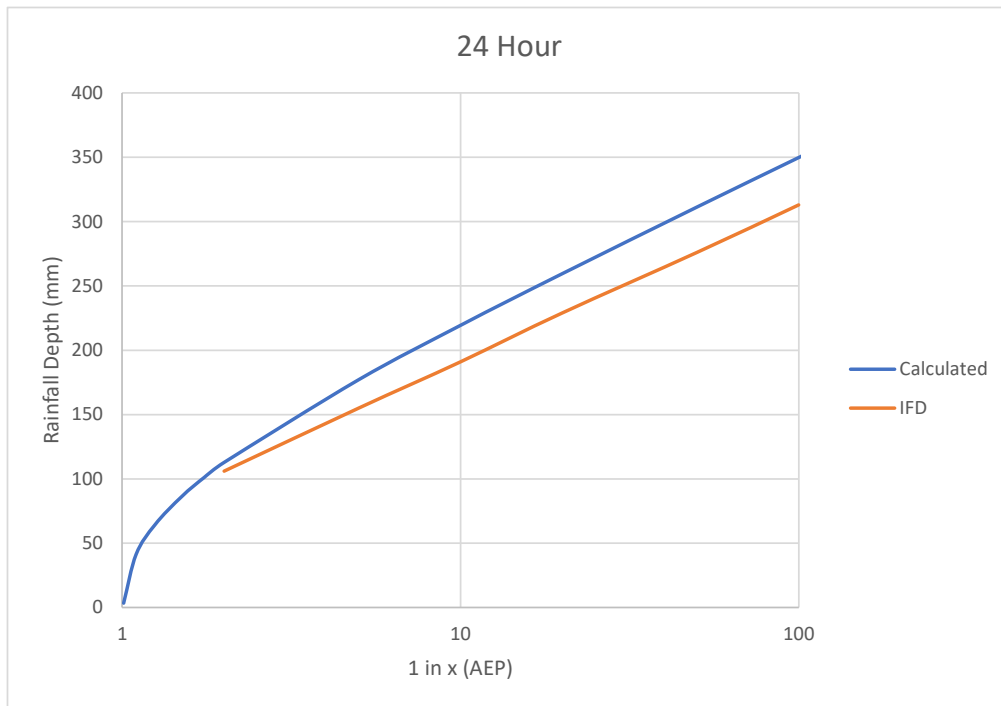
Figure D.10 Gauge 58032 (Kyogle Post Office), 24 hour duration
