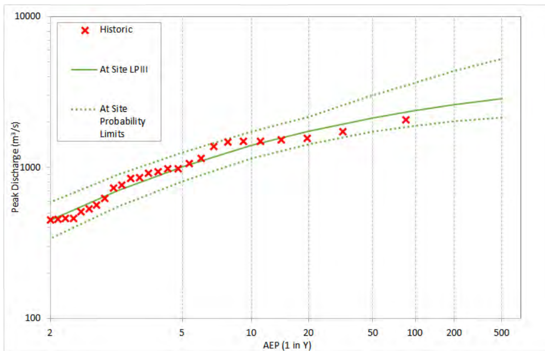
Figure 7.2 Flood Frequency Plot for Wiangaree
