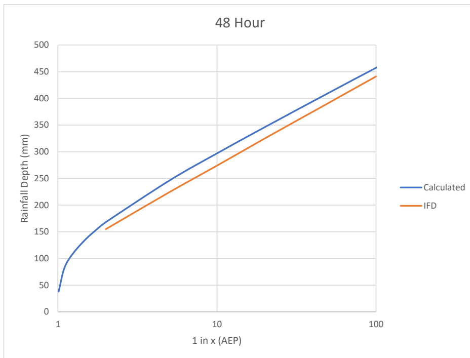
Figure D.13 Gauge 58097 (New Italy Vineyard Haven), 48 hour duration
