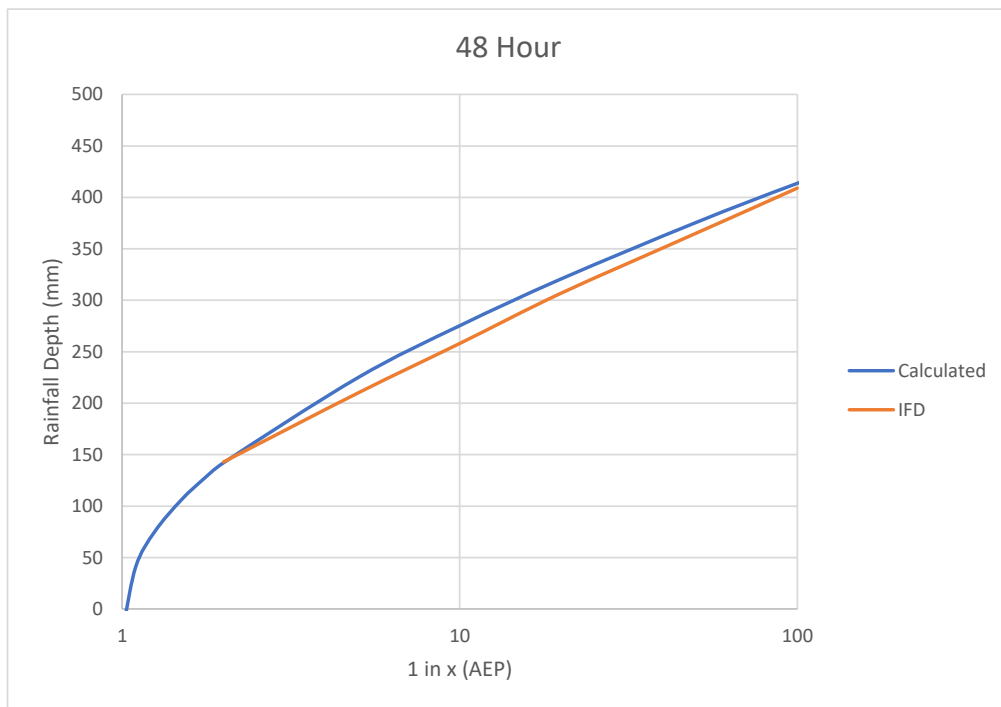
Figure D.11 Gauge 58032 (Kyogle Post Office), 48 hour duration
