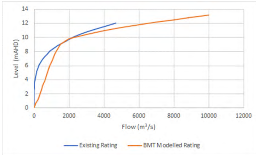
Figure 7.4 East Gundurimba Rating Curves
