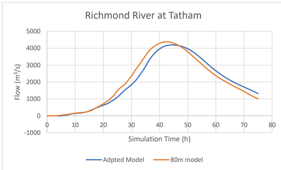
Figure F.2 Comparison at Tatham (24h storm duration)
