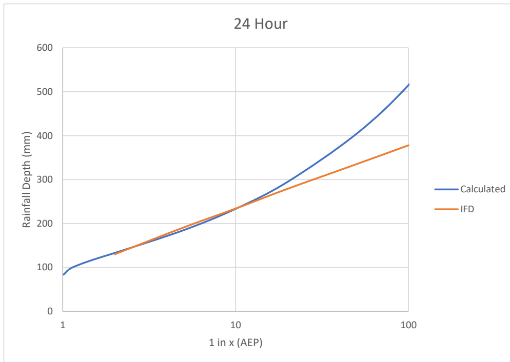
Figure D.14 Gauge 58147 (The Channon), 24 hour duration
