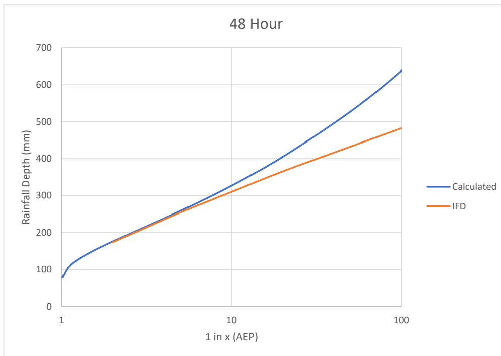
Figure D.15 Gauge 58147 (The Channon), 48 hour duration
