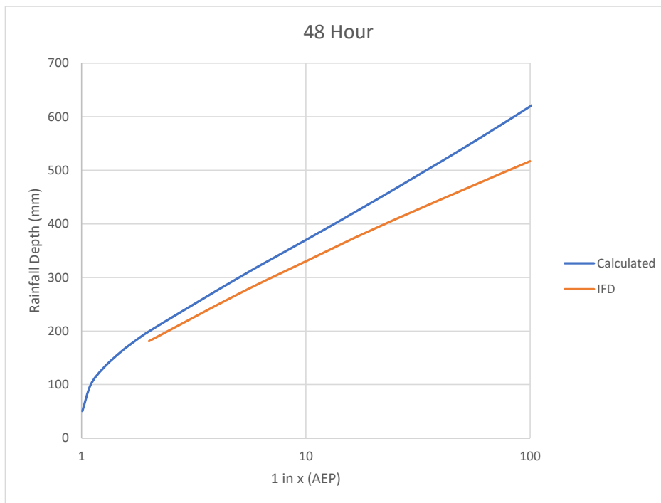
Figure D.9 Gauge 58044 (Nimbin Post Office), 48 hour duration
