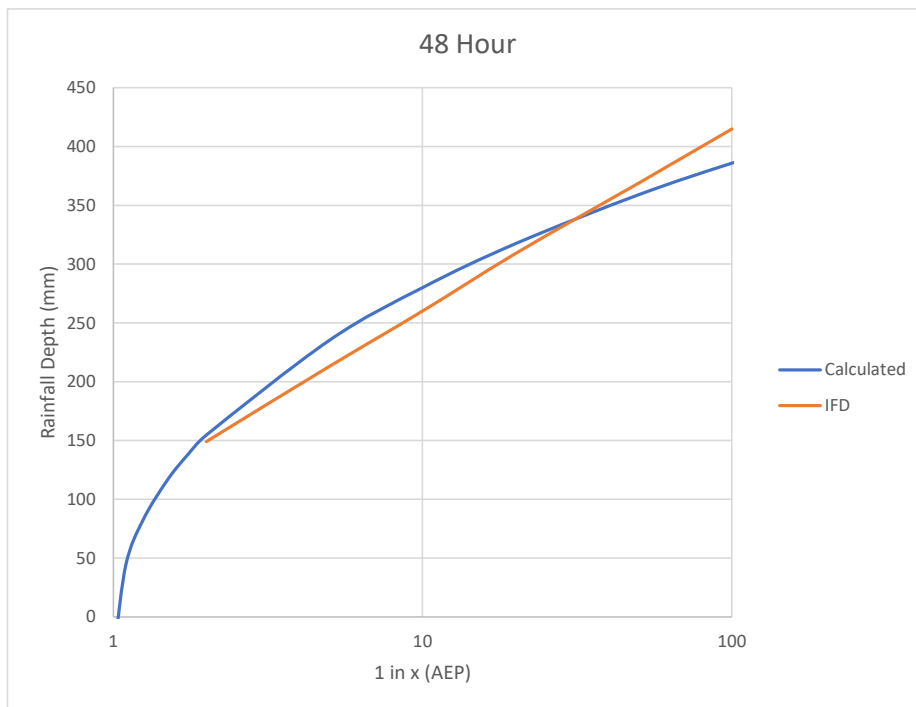
Figure D.19 Gauge 58004 (Mummulgum, Bingebeebebra), 48 hour duration
