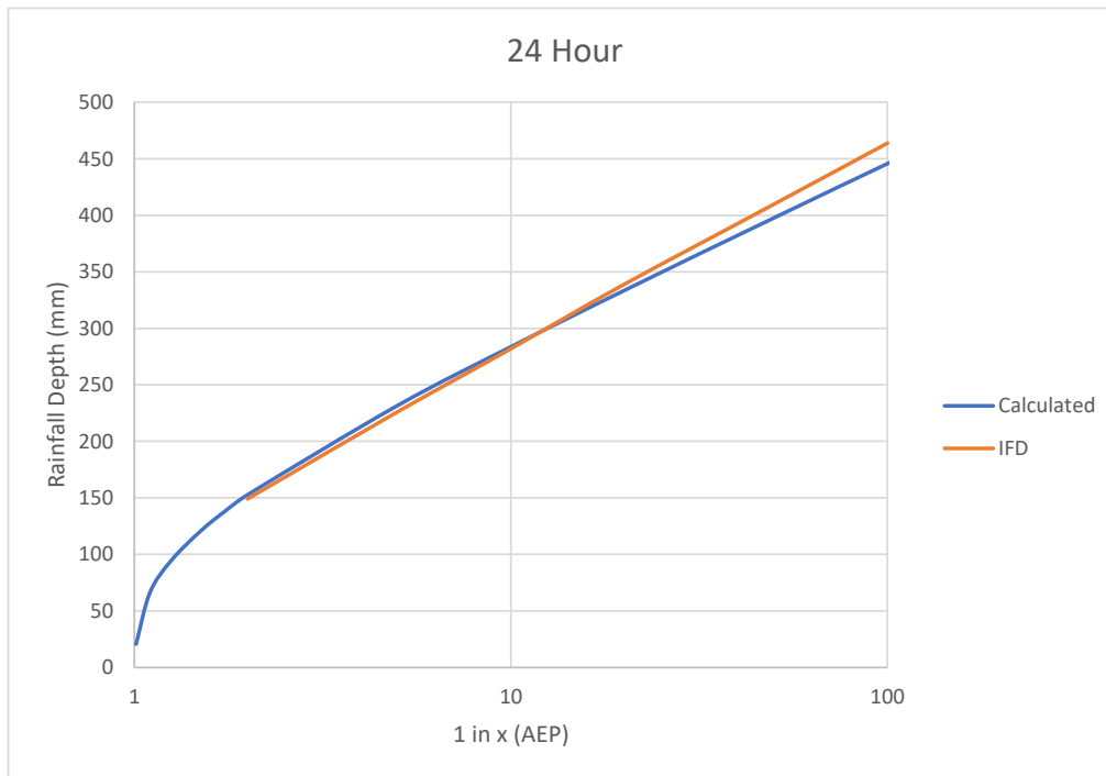
Figure D.24 Gauge 58148 (Lillian Rock, Williams Road), 24 hour duration
