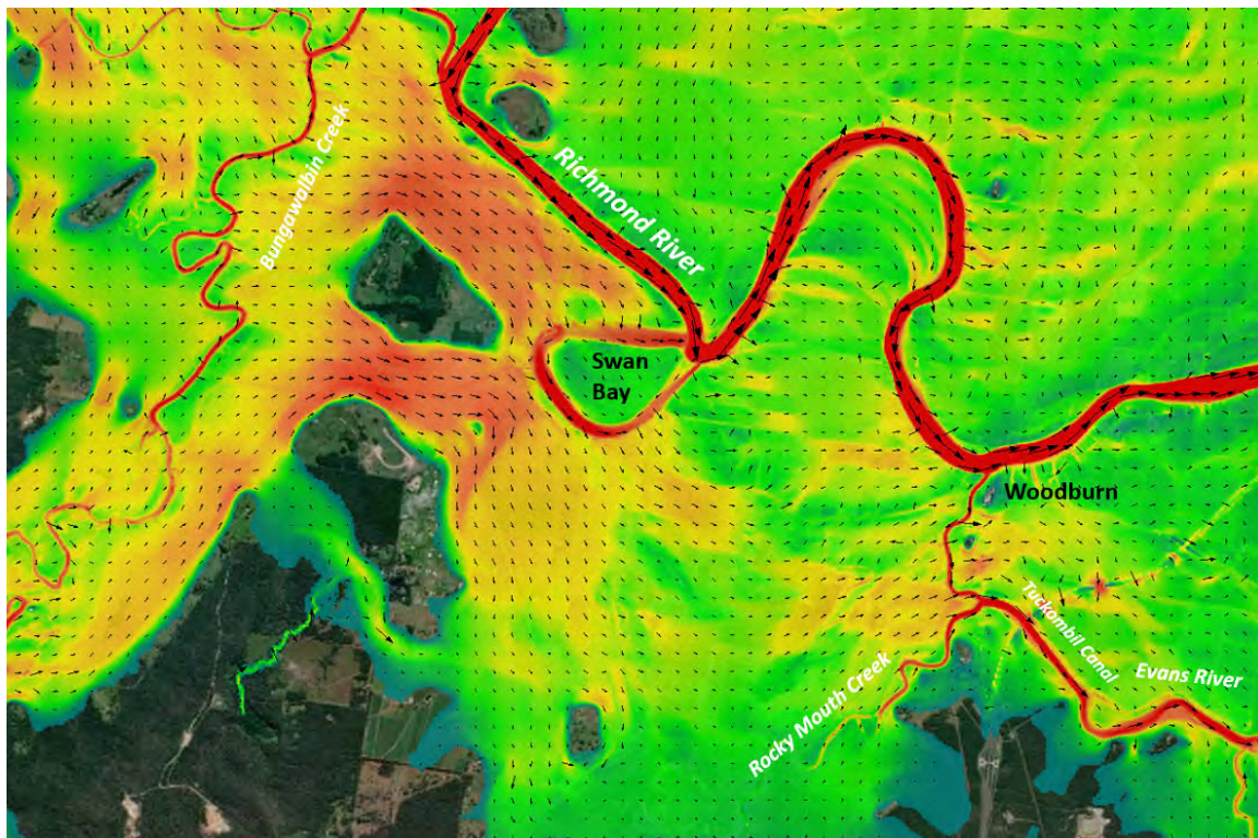
Figure 6.17 February/March 2022 Event showing interaction of flow in floodplain shown using velocity-depth product
