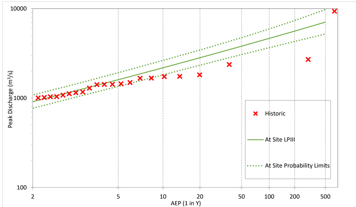
Figure 7.5 Flood Frequency Plot for east Gundurimba
