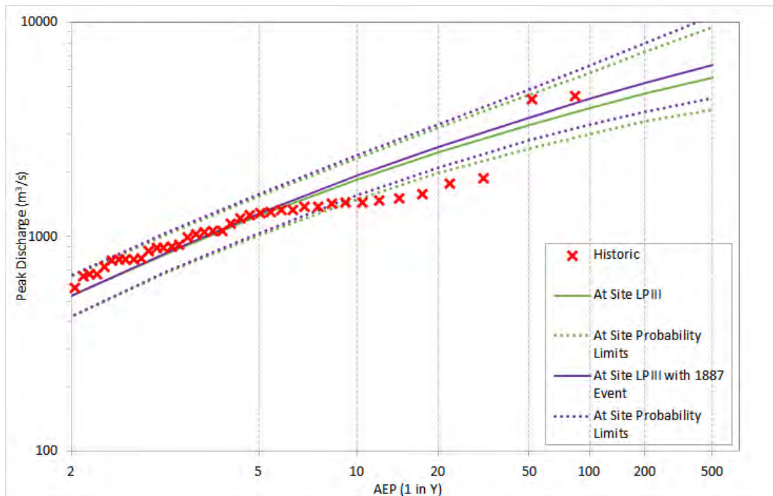
Figure 7.1 Flood Frequency Plot for Casino
