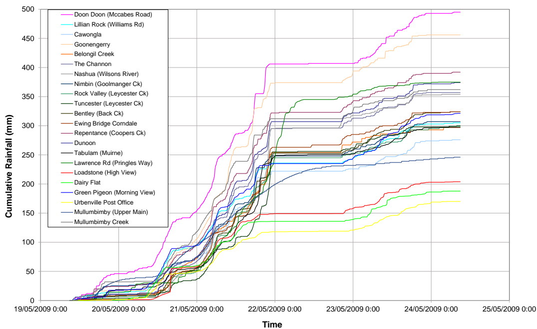
Figure 6.8 May 2009 Event: Cumulative Rainfall
