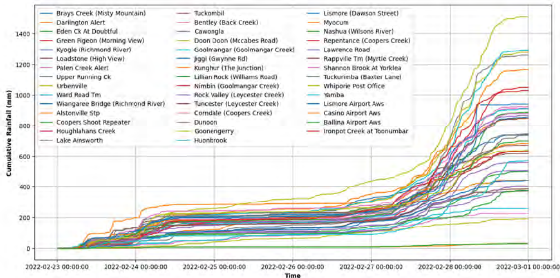
Figure 6.2 February/March 2022 Event: Cumulative Rainfall
