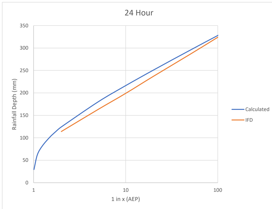
Figure D.18 Gauge 58004 (Mummulgum, Bingebeebebra), 24 hour duration
