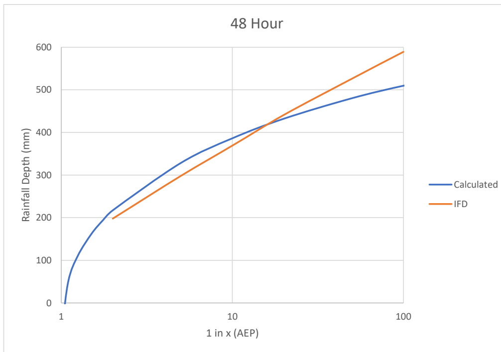
Figure D.29 Gauge 58113 (Green Pigeon, Morning View), 48 hour duration
