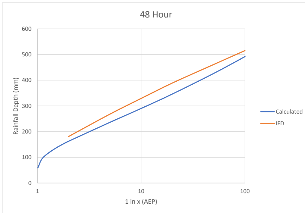
Figure D.5 Gauge 58180 (Nimbin, Goolmangar Creek), 48 hour duration
