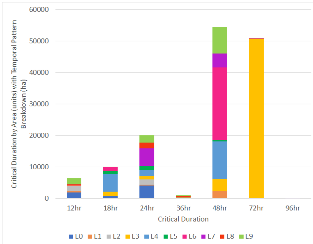
Figure 8.9 Graphical Representation of Event Selection: 0.2% AEP
