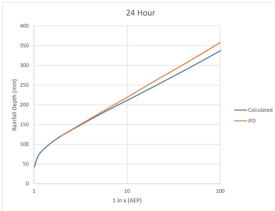
Figure D.2 Gauge 58061 (Woodburn, Cedar Street), 24 hour duration
