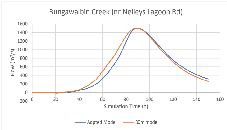
Figure F.4 Comparison on Bungawalbin Creek (72h storm duration)
