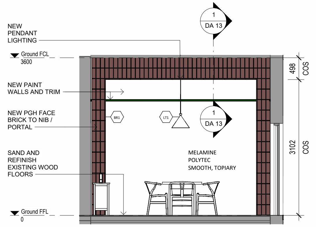
4 FUNCTION ELEVATION 1 : 50
