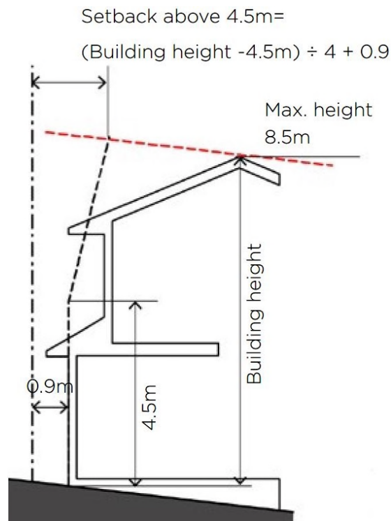
Figure 8: Side Boundary Setback Calculation
