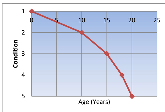
Figure 7-4: Road Decay Curve
